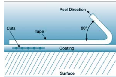
Position of the adhesive tape before peeling it off the cross-cut surface
